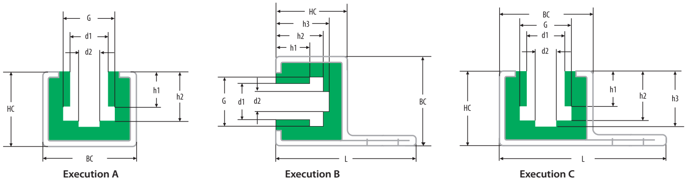
Execution A - Suitable for galvanized or stainless steel channel.
